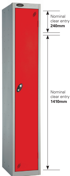
1 compartment Fixed top shelf with double coat hook.
