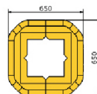
Top Profile
